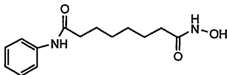
Suberoylanilide Hydroxamic Acid (SAHA)
